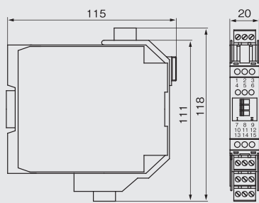
KFD2-SR2-Ex1.W.LB
