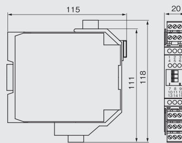
KFD2-SR2-Ex2.W
