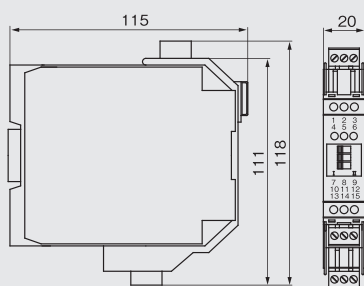
KFD2-SR2-Ex1.W
